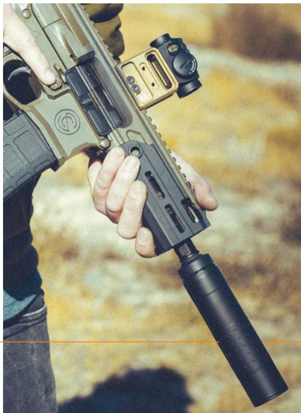
Chimera 300 with 3-Lug Mount and Charlie Flat Front Cap, Sig Rattler
